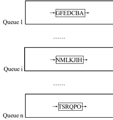
Figure 4: Algorithm principle
