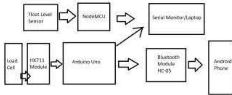
Fig. 1 Block schematic
